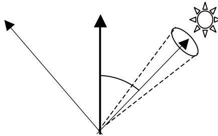
Figure 5. BRDF
