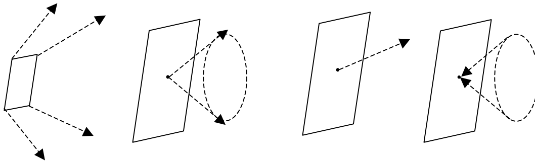
Figure 1. Radiometric quantities
