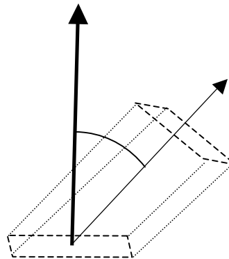
Figure 3. Projected area
