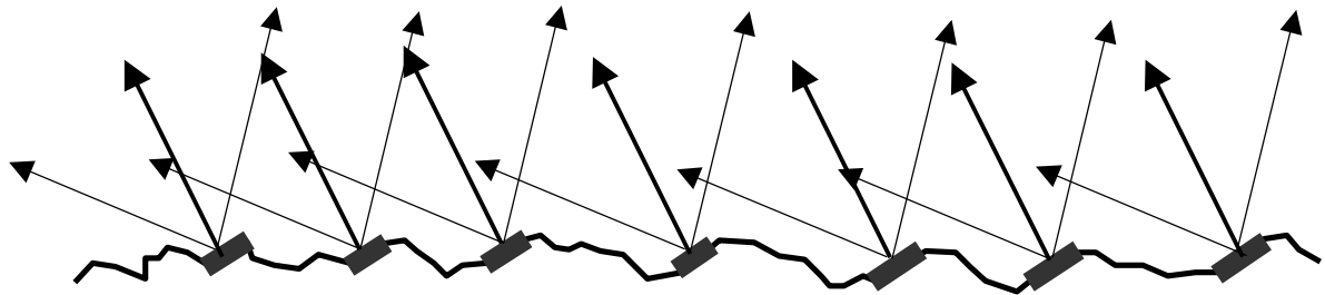
Figure 6. Micro-facets
